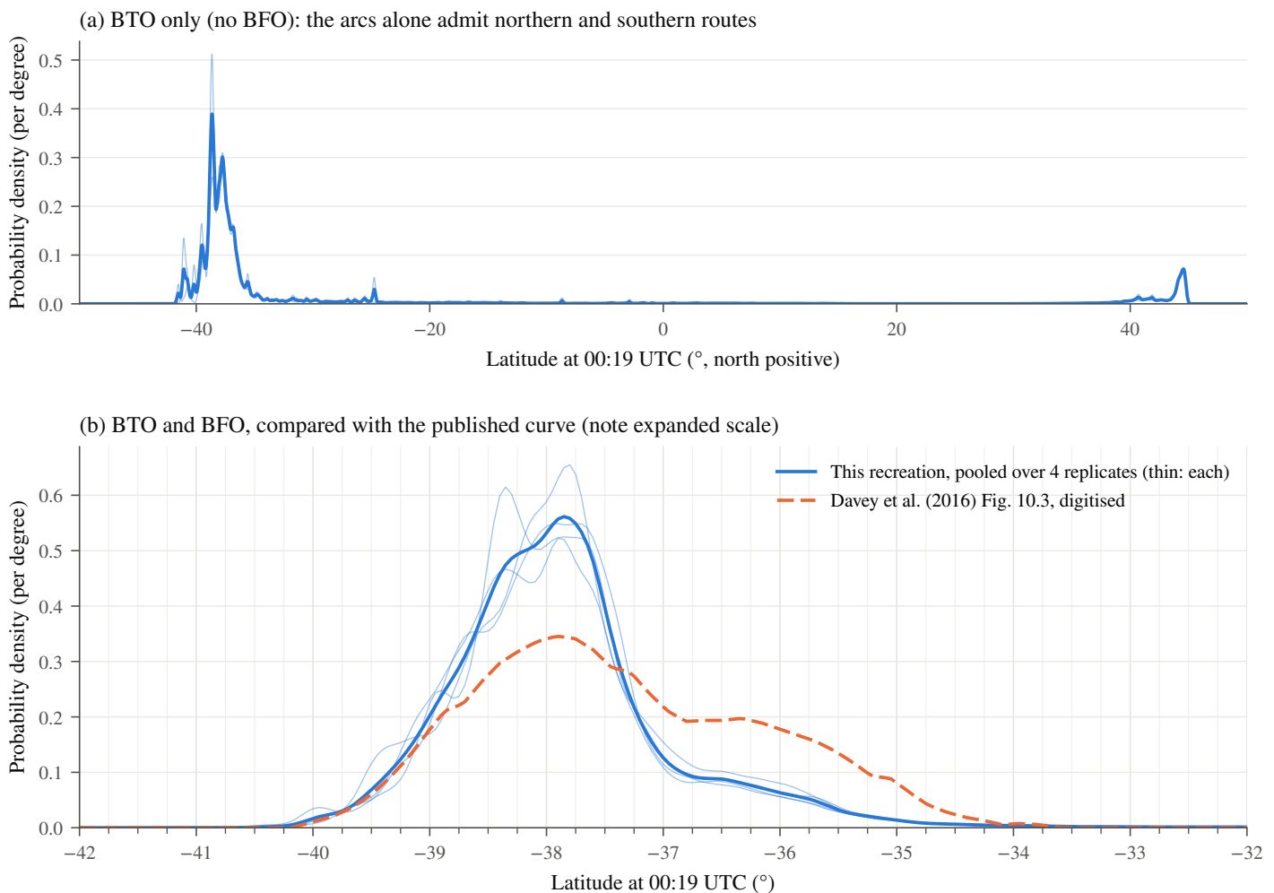
Figure 1. Latitude pdf of the aircraft at 00:19:37 UTC, the form of Davey et al. Fig. 10.3. (a) BTO only. (b) BTO and BFO, with the published curve. Densities are weighted particle histograms smoothed with a 0.1° Gaussian; each particle carries its own altitude. Evidence: BTO at every epoch except the 18:39 and 23:15 C-channel calls; BFO (bottom only) at 18:28, 18:39, 19:41–22:41, 23:15 and 00:11. No fuel, debris, drift, search or end-of-flight evidence is used. Run 'davey-inmarsat-baseline' is not the base configuration, but no --baseline was given, so the differences from it are not stated here.
